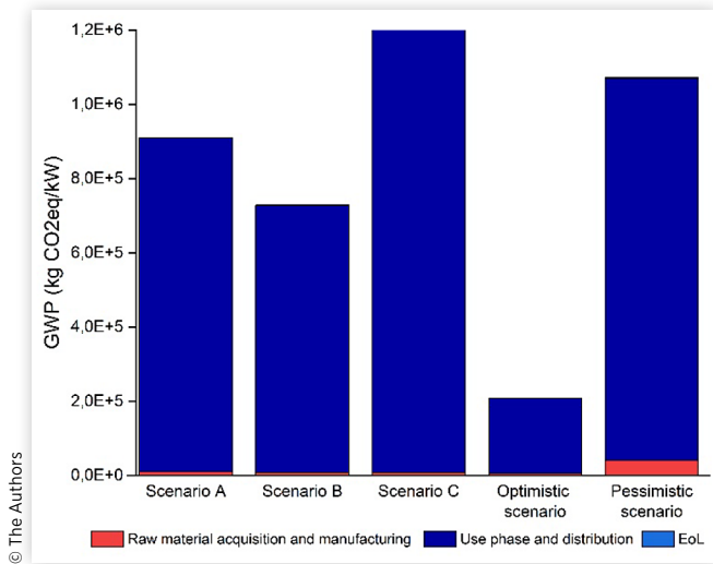
FIGURE 3 Climate change results for the cradle-to-grave boundary
