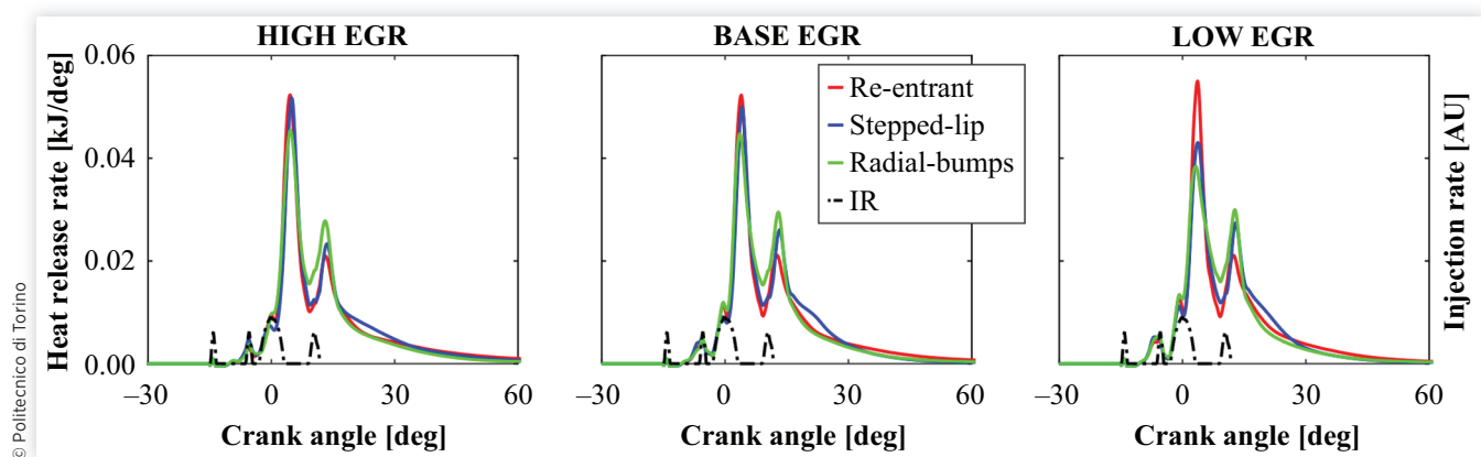
FIGURE 11 HRR for the EGR sweep and partial-load injection rate profile. Engine operating condition: 1500 RPM \times 5.0 bar BMEP.
